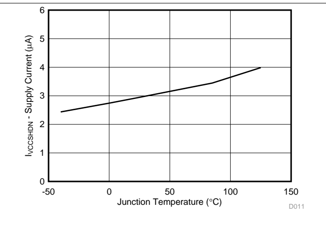
Figure 11. VIN Shutdown Current vs Junction Temperature
