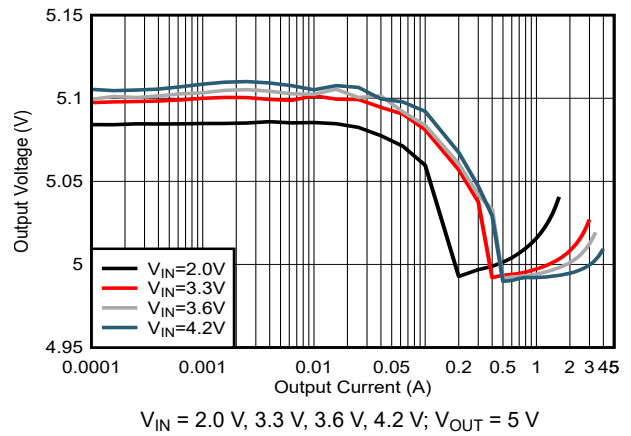
Figure 6-4. Load Regulation in Auto PFM
