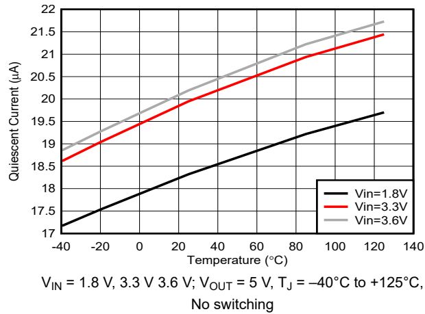
Figure 6-7. Quiescent Current into VIN vs Temperature
