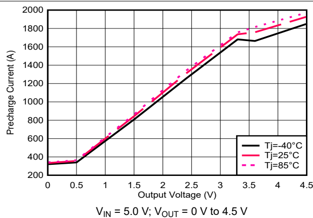
Figure 6-5. Pre-charge Current vs Output Voltage
