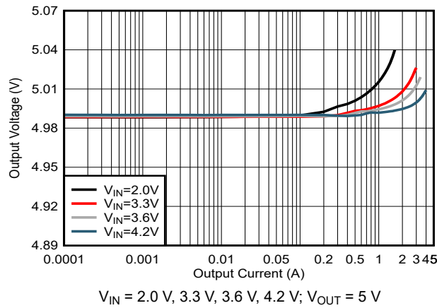
Figure 6-3. Load Regulation in Forced PWM
