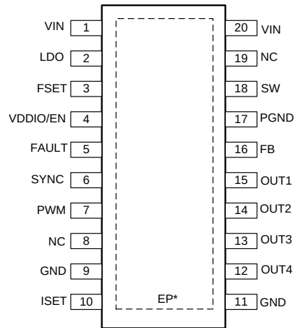
PWP Package 20-Pin HTSSOP With Exposed Thermal Pad Top View
