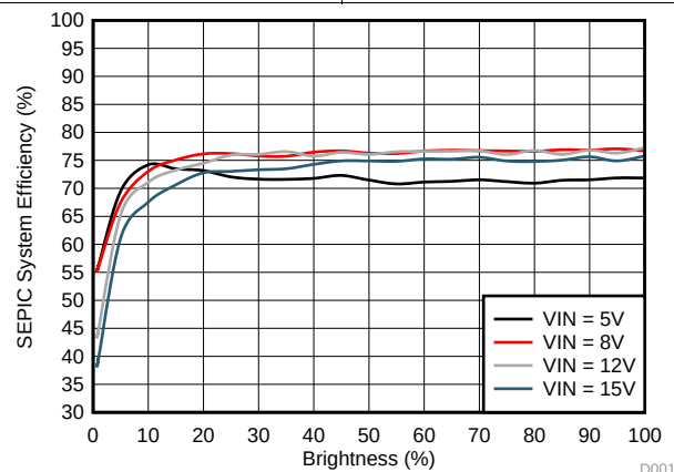
Figure 26. SEPIC Efficiency
