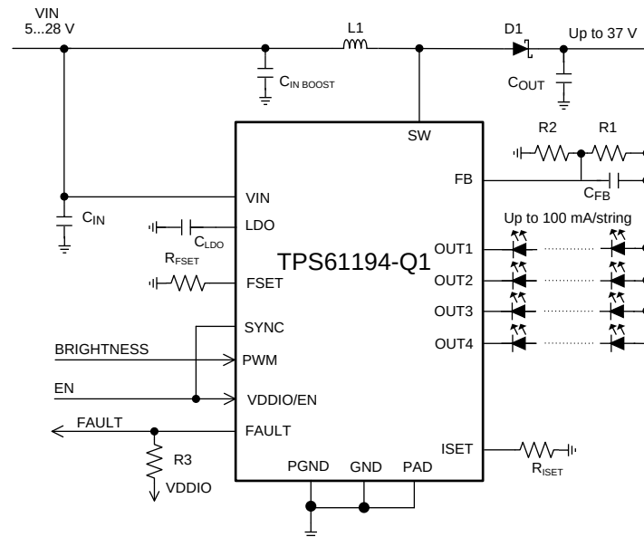
Figure 20. Four Strings 80 mA per String Configuration
