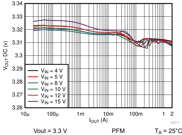
Figure 10-26. Output Voltage vs Output Current
