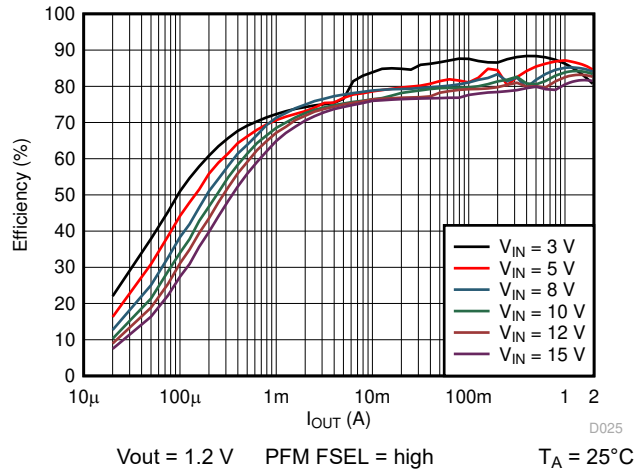
Figure 10-2. Efficiency vs Output Current
