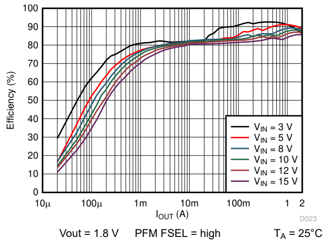
Figure 10-6. Efficiency vs Output Current
