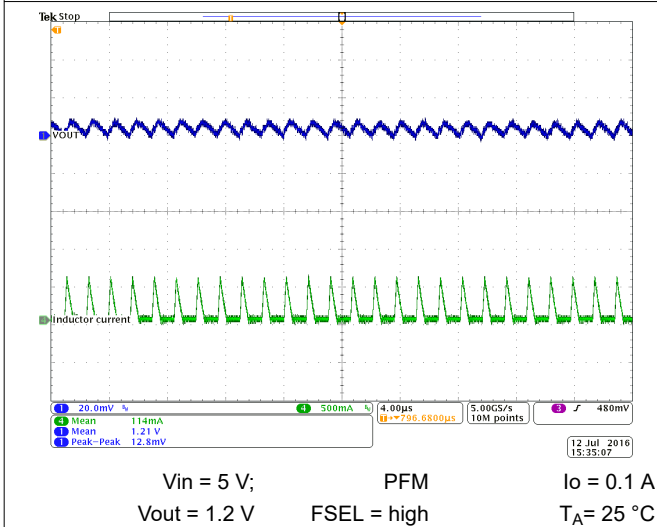
Figure 10-36. Output Voltage Ripple
