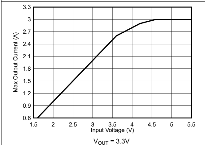
Figure 8-6. Typical Output Current Capability vs Input Voltage
