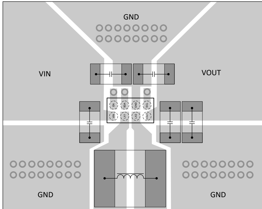
Figure 8-24. Layout Example
