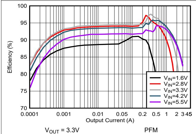
Figure 8-4. Efficiency vs Input Voltage (PFM)
