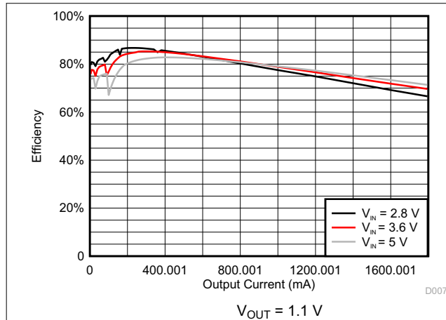
Figure 8-2. DCDC1/DCDC2 Efficiency
