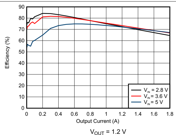
Figure 8-3. DCDC3 Efficiency
