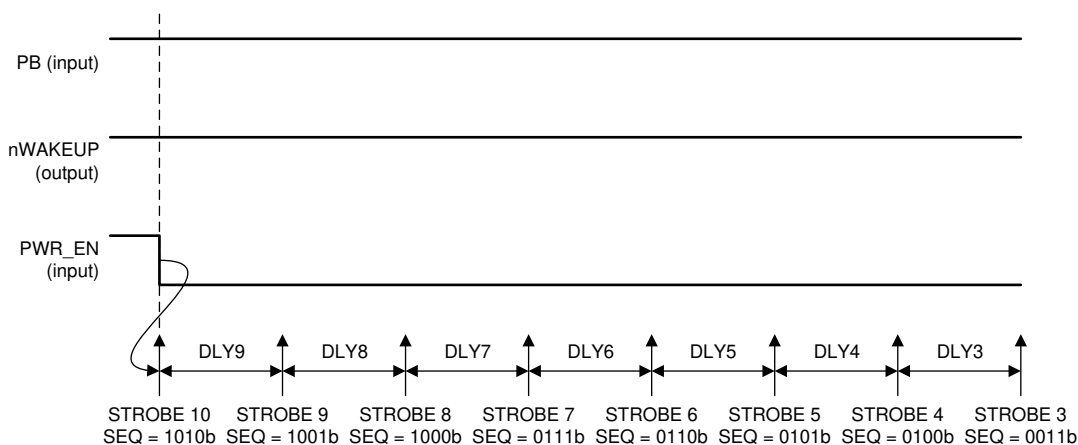
Figure 6-4. Power-Down Sequences to OFF State; PWR_EN is Power-Down Event
