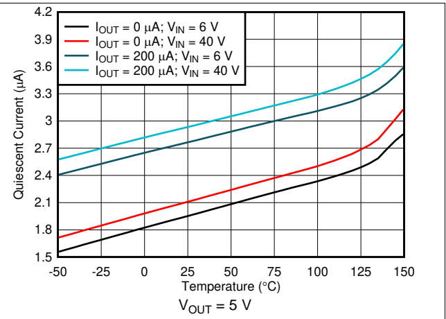
Figure 2. Quiescent Current vs Ambient Temperature
