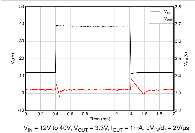
Figure 5-45. Line Transient (12V to 40V)
