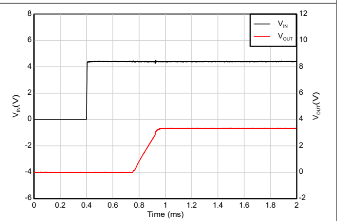
Figure 5-32. Start-up with EN & V_{IN} tied together
