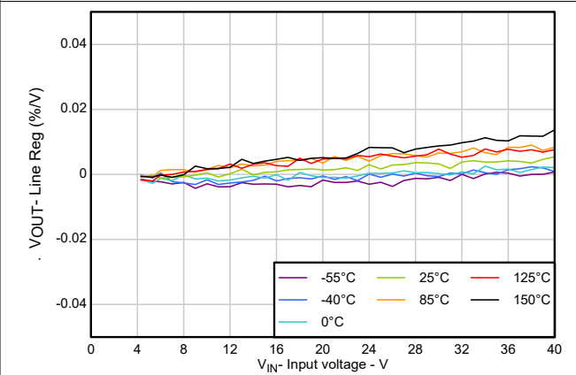
Figure 5-4. Line Regulation
