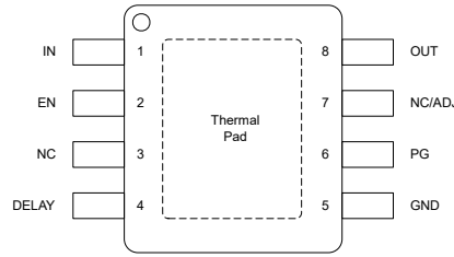
Figure 4-3. DGN Package (Fixed/ADJ), 8-Pin HVSSOP (Top View)
