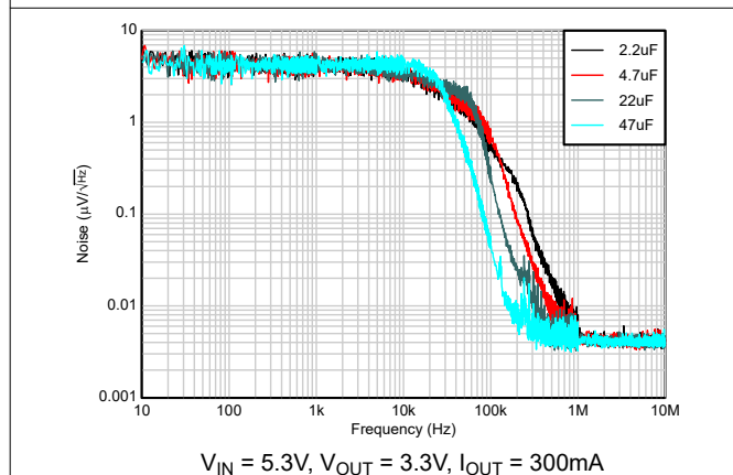
Figure 5-23. Output Noise vs Frequency, C_{OUT}
