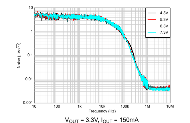
Figure 5-24. Output Noise vs Frequency, Input Voltage
