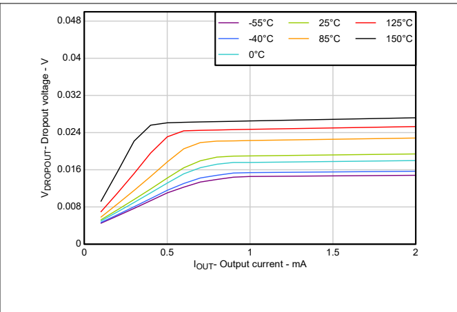
Figure 5-8. Dropout Voltage vs Output Current, Light Loads
