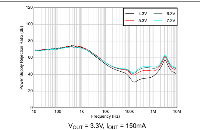
Figure 5-20. Ripple Rejection vs Frequency, Input Voltage
