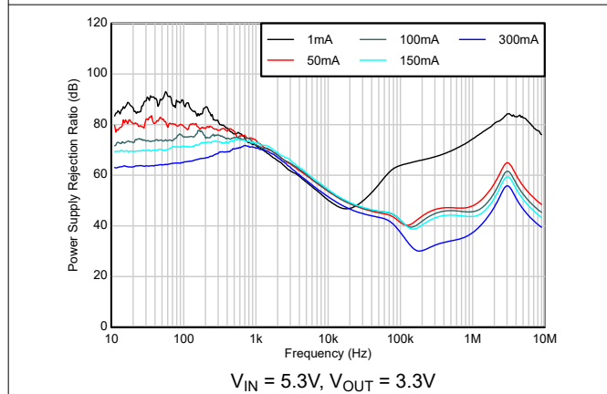
Figure 5-21. Ripple Rejection vs Frequency, Output Current
