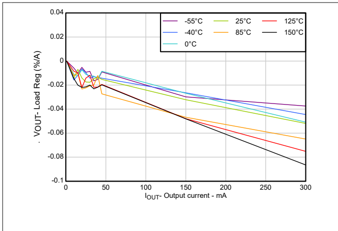
Figure 5-7. Load Regulation vs Output Current
