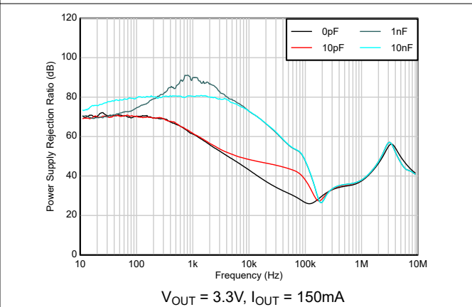
Figure 5-22. Ripple Rejection vs Frequency, C_{FF}
