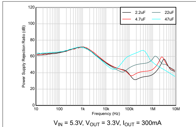
Figure 5-19. Ripple Rejection vs Frequency, C_{OUT}
