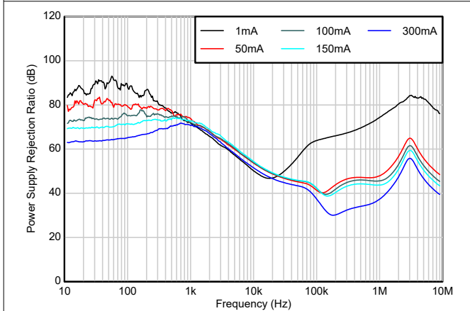
Figure 5-19. PSRR vs I_{OUT}
