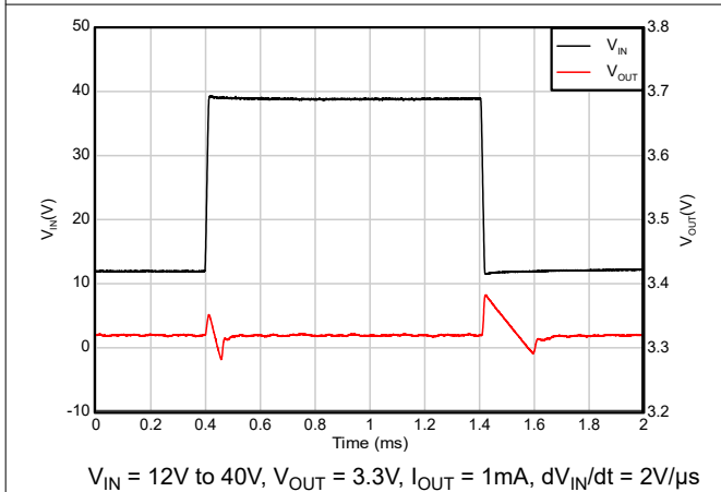
Figure 5-37. Line Transient (12V to 40V)
