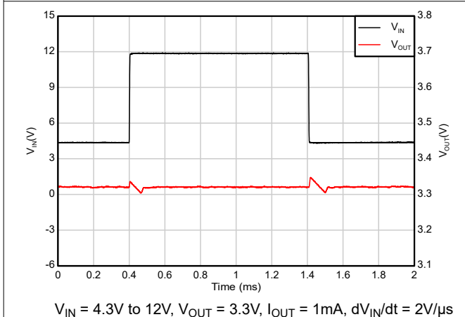
Figure 5-35. Line Transient (4.3V to 12V)
