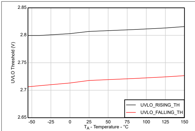
Figure 5-17. UVLO Threshold ( V_{UVLO+}/V_{UVLO-} ) vs Temperature
