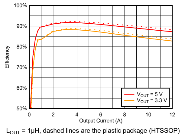
Figure 7-6. Efficiency vs Load Across VOUT at V_{IN} = 12V , 1MHz
