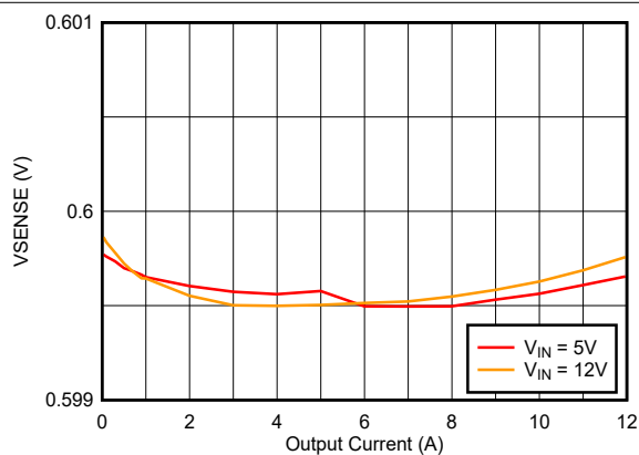
Figure 7-33. V_{SENSE} vs Output Current at 1MHz
