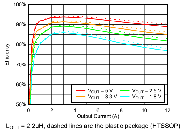
Figure 7-4. Efficiency vs Load Across VOUT at V_{IN} = 12V , 500kHz
