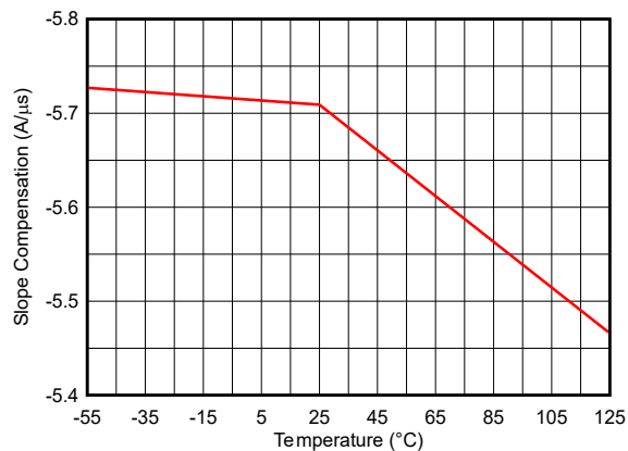
Figure 7-43. Slope Compensation vs Temperature at 100kHz
