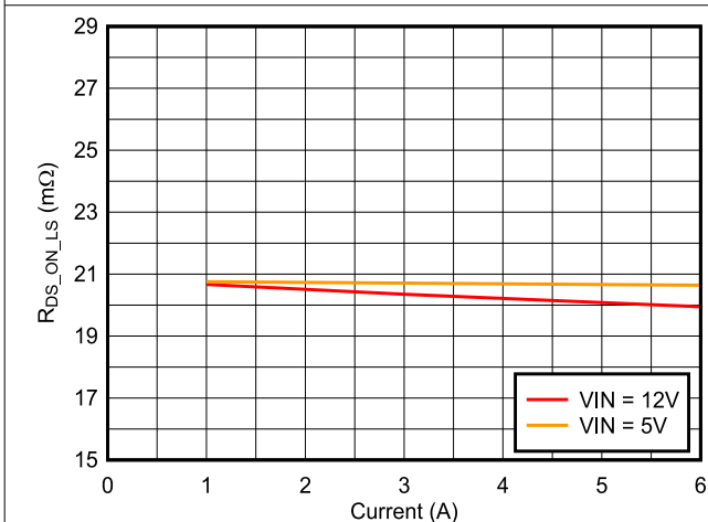
Figure 7-53. Low Side FET Resistance vs Current
