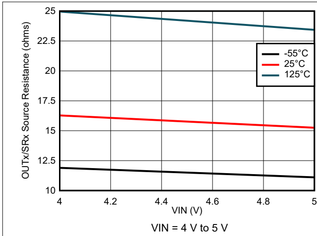
Figure 7-61. Output Source Resistance Variation
