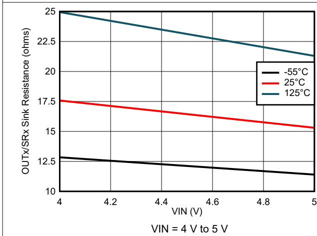
Figure 7-63. Output Sink Resistance Variation
