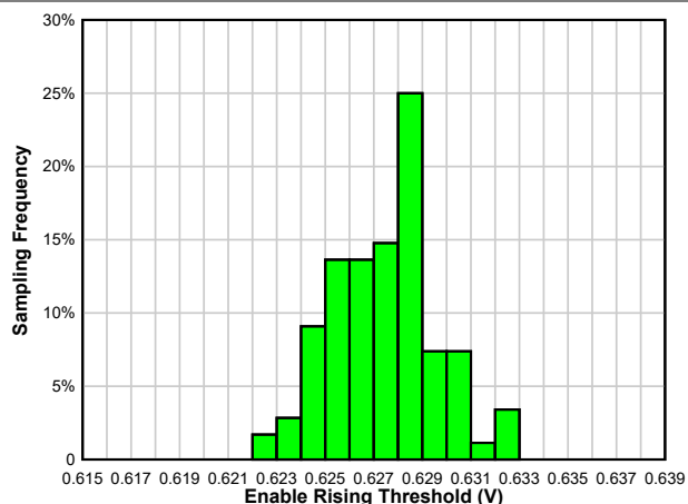
Figure 6-42. Enable Rising Threshold Distribution at T_A = 25^\circ\text{C}
