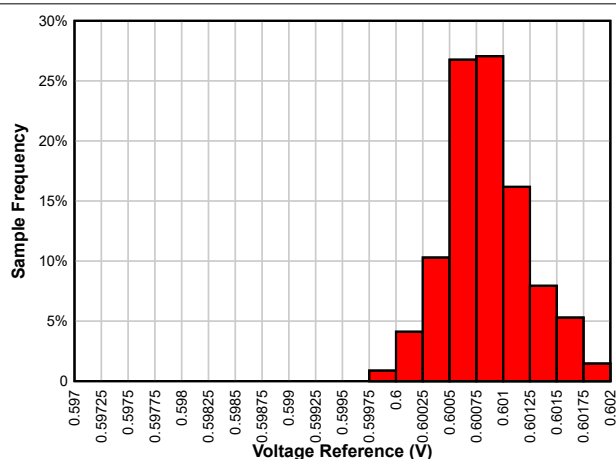
Figure 6-50. Voltage Reference Distribution at T_A = -55^{\circ}\text{C}
