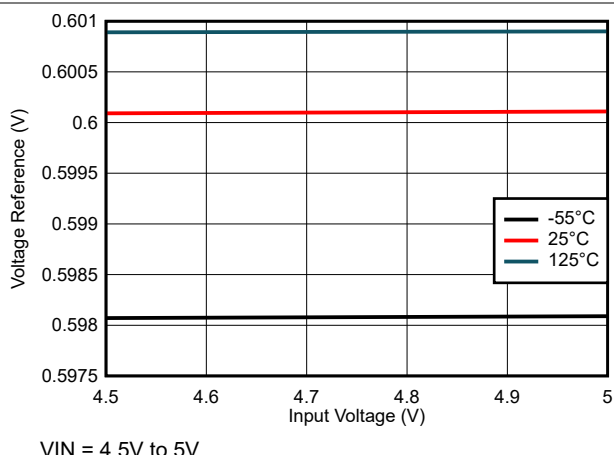
Figure 6-20. Internal Voltage Reference vs Input Voltage
