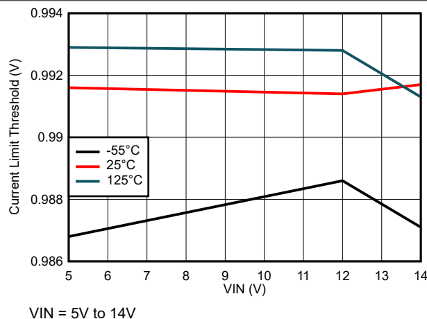
Figure 6-23. Current Limit Threshold vs Input Voltage
