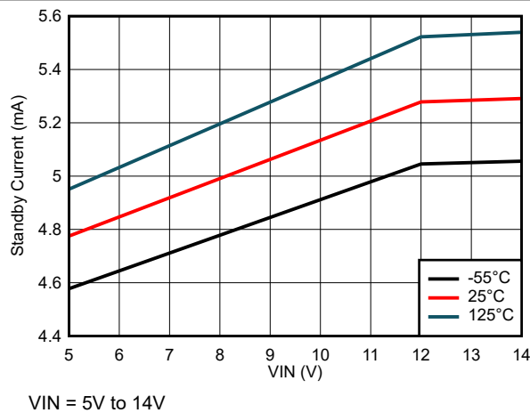
Figure 6-33. Standby Current vs Input Voltage
