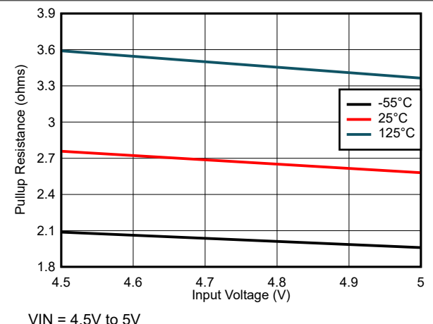
Figure 6-24. Pullup Resistance vs Input Voltage
