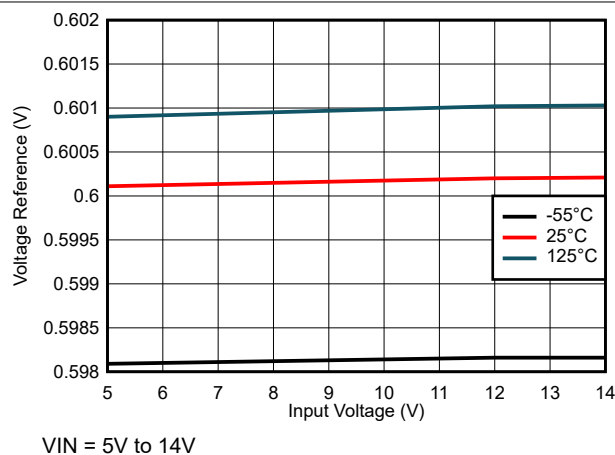
Figure 6-21. Internal Voltage Reference vs Input Voltage
