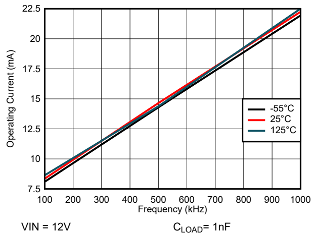
Figure 6-31. Operating Supply Current vs Frequency
