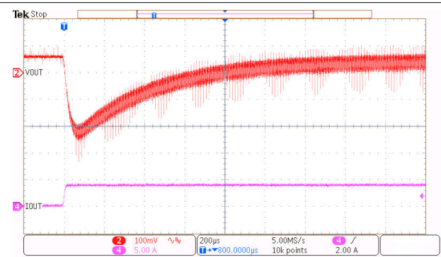
Figure 8-3. 4A Load Step Response for Flyback Converter
