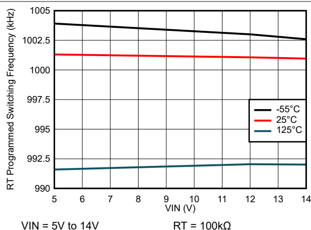
Figure 6-19. Switching Frequency vs Input Voltage
