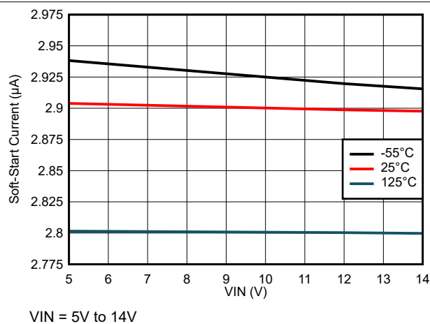
Figure 6-35. Soft-Start Current vs Input Voltage
