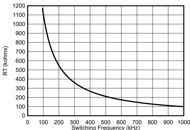
Figure 7-8. RT vs Switching Frequency
