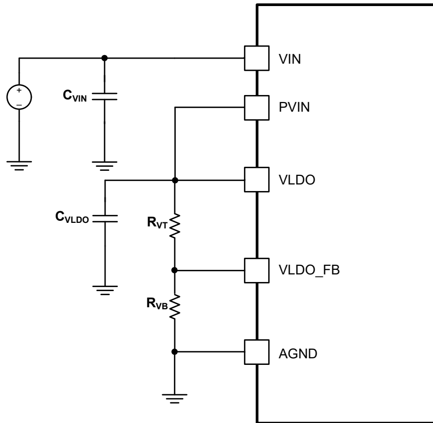
Figure 7-5. Configuration for PVIN to VLDO Connection for TPS7H502x
