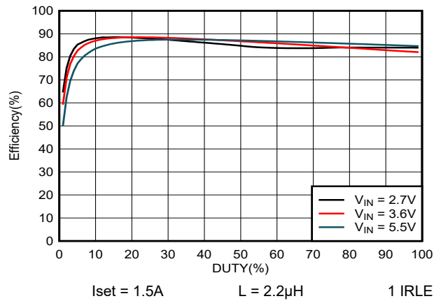
Figure 8-2. 1 IRLED Output Efficiency
