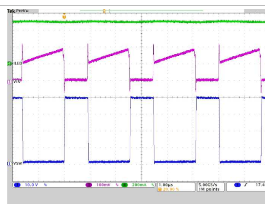
Ch1: Switch node voltage; Ch3: Switch sense resistor voltage; Ch4: LED current; Time: 1 μs/div Figure 34. Normal Operation
