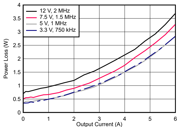
Figure 7-15. Power Dissipation
