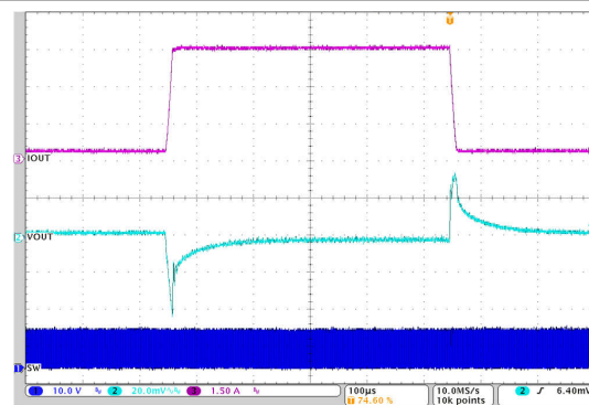
Figure 7-17. Load Transient
