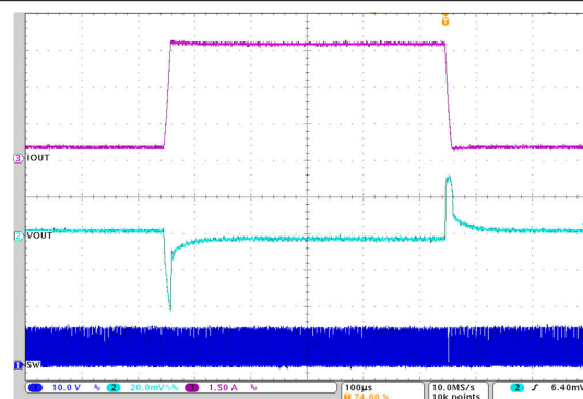
Figure 7-15. Load Transient
