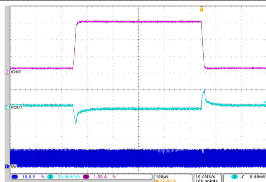
Figure 7-14. Load Transient
