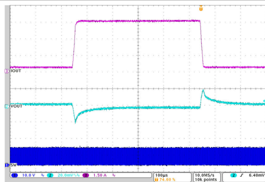
Figure 7-16. Load Transient
