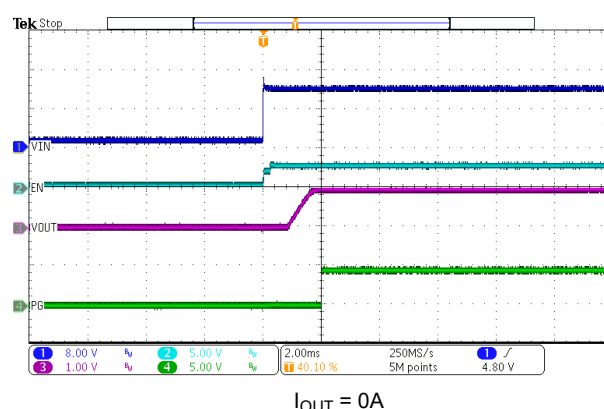
Figure 7-13. VIN Start-Up
