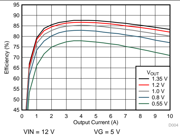
Figure 2. Efficiency
