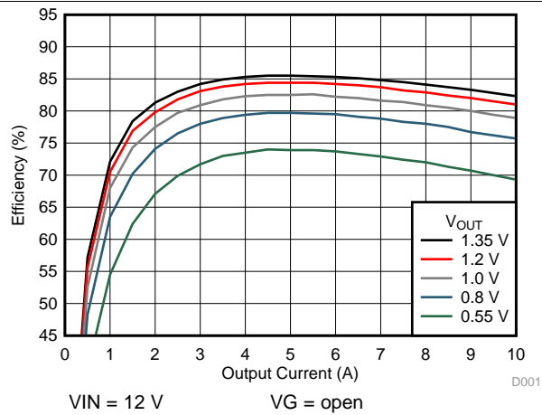
Figure 1. Efficiency
