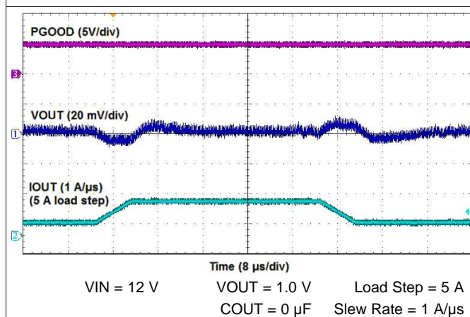
Figure 13. Transient Response
