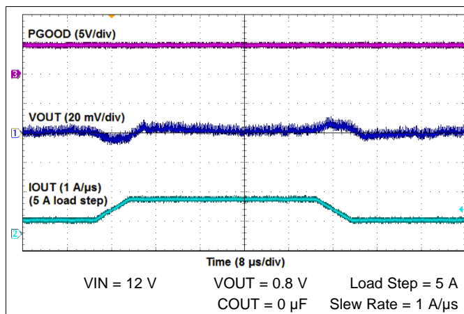
Figure 11. Transient Response
