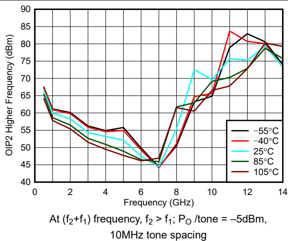
Figure 5-21. OIP2 Higher Across Temperature
