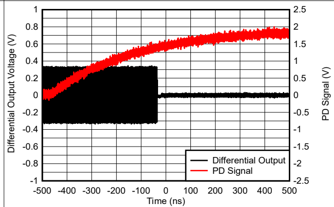
Figure 5-48. Step Response
