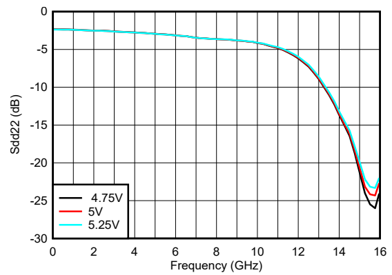
P_{IN} = -20\text{dBm} with 50Ω source at all excited ports, nonexcited ports are terminated with 50Ω
