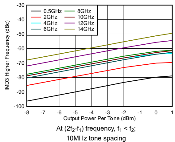
Figure 5-18. IMD3 Higher Across Output Power
