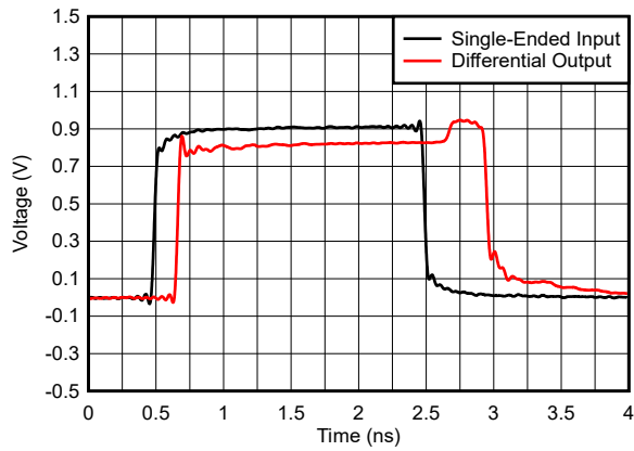
Figure 5-47. Overdrive Recovery Response
