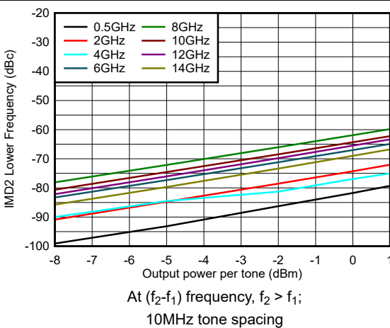
Figure 5-27. IMD2 Lower Across Output Power
