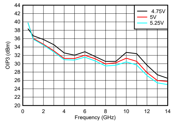
P_O / \text{tone} = -5\text{dBm} , 10MHz tone spacing
