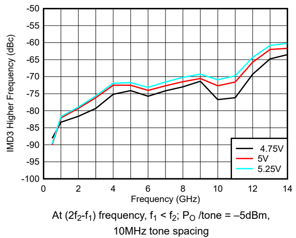
Figure 5-16. IMD3 Higher Across V_{DD}
