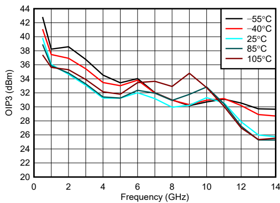
P_O / \text{tone} = -5\text{dBm} , 10MHz tone spacing
