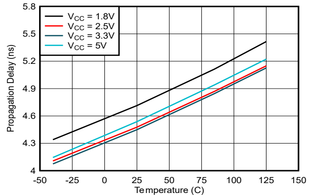
Figure 5-6. Propagation Delay, T_{PLH} , vs Temperature
