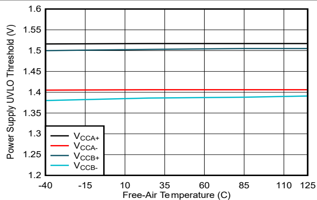
Figure 5-8. Power Supply Undervoltage Threshold vs Free-Air Temperature
