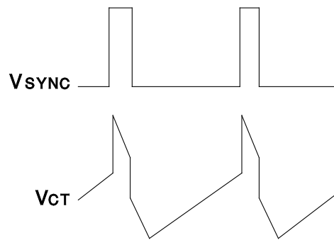
Figure 7-8. Operational Waveforms
