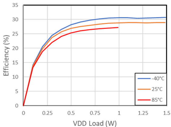
Figure 7-18. Efficiency vs. Load on V_{VDD-VEE} : V_{IN} = 18 V, V_{VDD-VEE} = 22 V, V_{COM-VEE} = 4 V, No Load on V_{COM-VEE}
