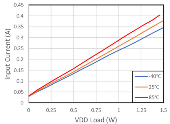
Figure 7-19. Input Current vs. Load on V_{VDD-VEE} : V_{IN} = 9 V, V_{VDD-VEE} = 22 V, V_{COM-VEE} = 4 V, No Load on V_{COM-VEE}
