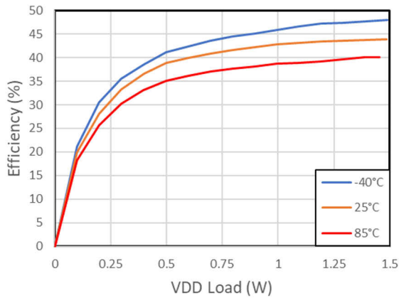
Figure 7-16. Efficiency vs. Load on V_{VDD-VEE} : V_{IN} = 9 V, V_{VDD-VEE} = 22 V, V_{COM-VEE} = 4 V, No Load on V_{COM-VEE}
