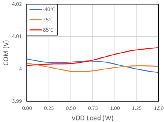
Figure 7-14. V_{COM-VEE} Load Regulation: V_{IN} = 12 V, V_{VDD-VEE} = 22 V, V_{COM-VEE} = 4 V
