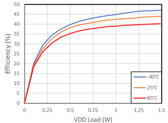
Figure 7-17. Efficiency vs. Load on V_{VDD-VEE} : V_{IN} = 12 V, V_{VDD-VEE} = 22 V, V_{COM-VEE} = 4 V, No Load on V_{COM-VEE}
