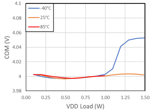
Figure 7-15. V_{COM-VEE} Load Regulation: V_{IN} = 18 V, V_{VDD-VEE} = 22 V, V_{COM-VEE} = 4 V
