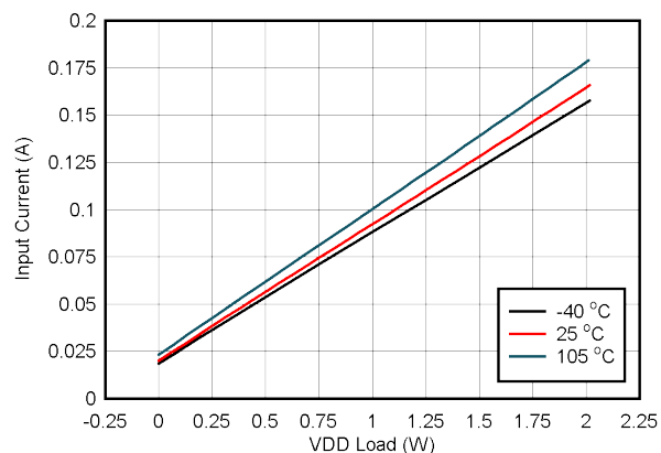
Figure 6-18. Input Current vs Load on V_{DDE-VEE} : V_{IN} = 21\text{ V} , V_{DDE-VEE} = 25\text{ V} , V_{COM-VEE} = 5\text{ V} , No Load on V_{COM-VEE}
