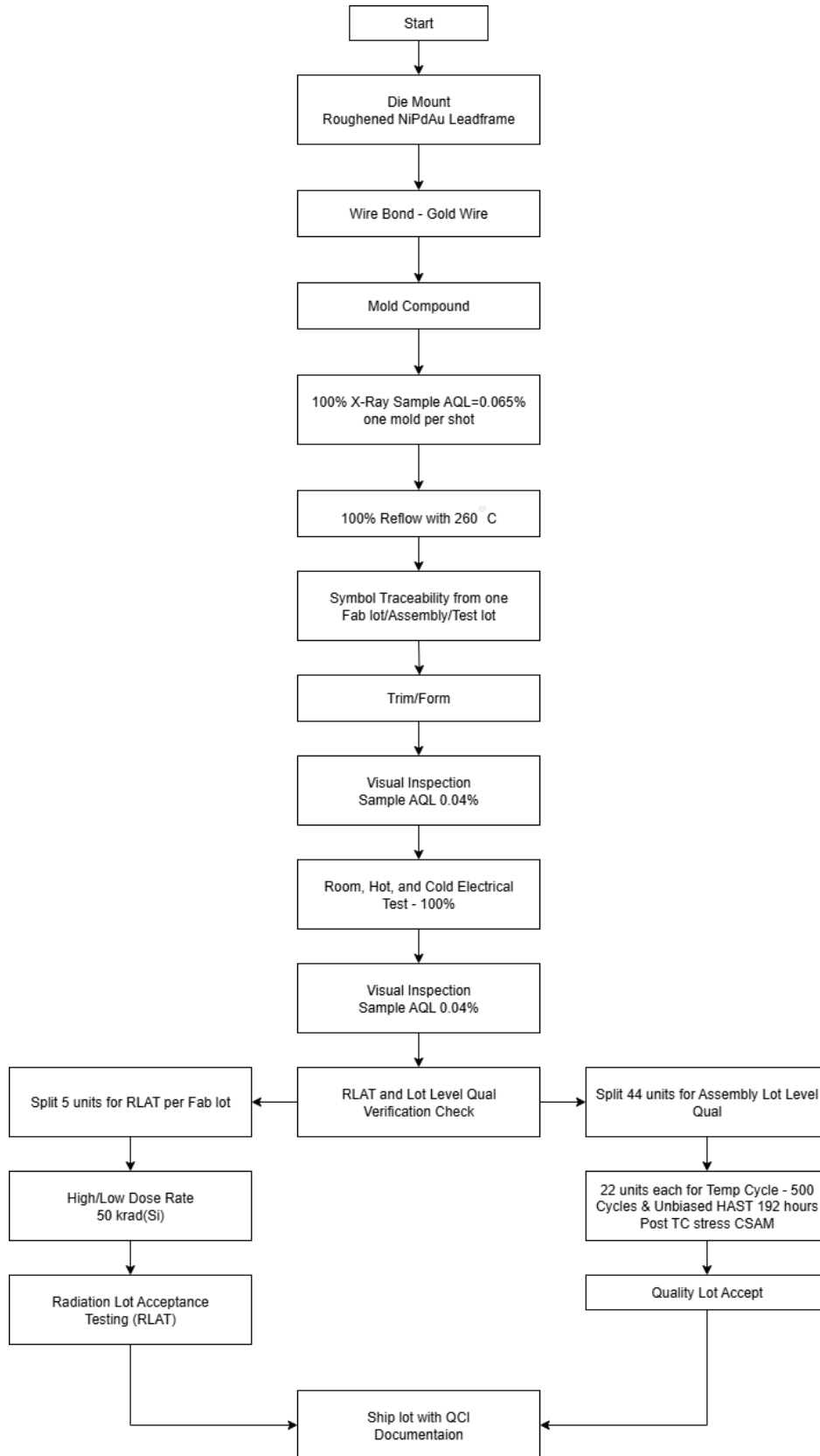
Figure 2-1. Space Enhanced Plastic Production Flow Chart
