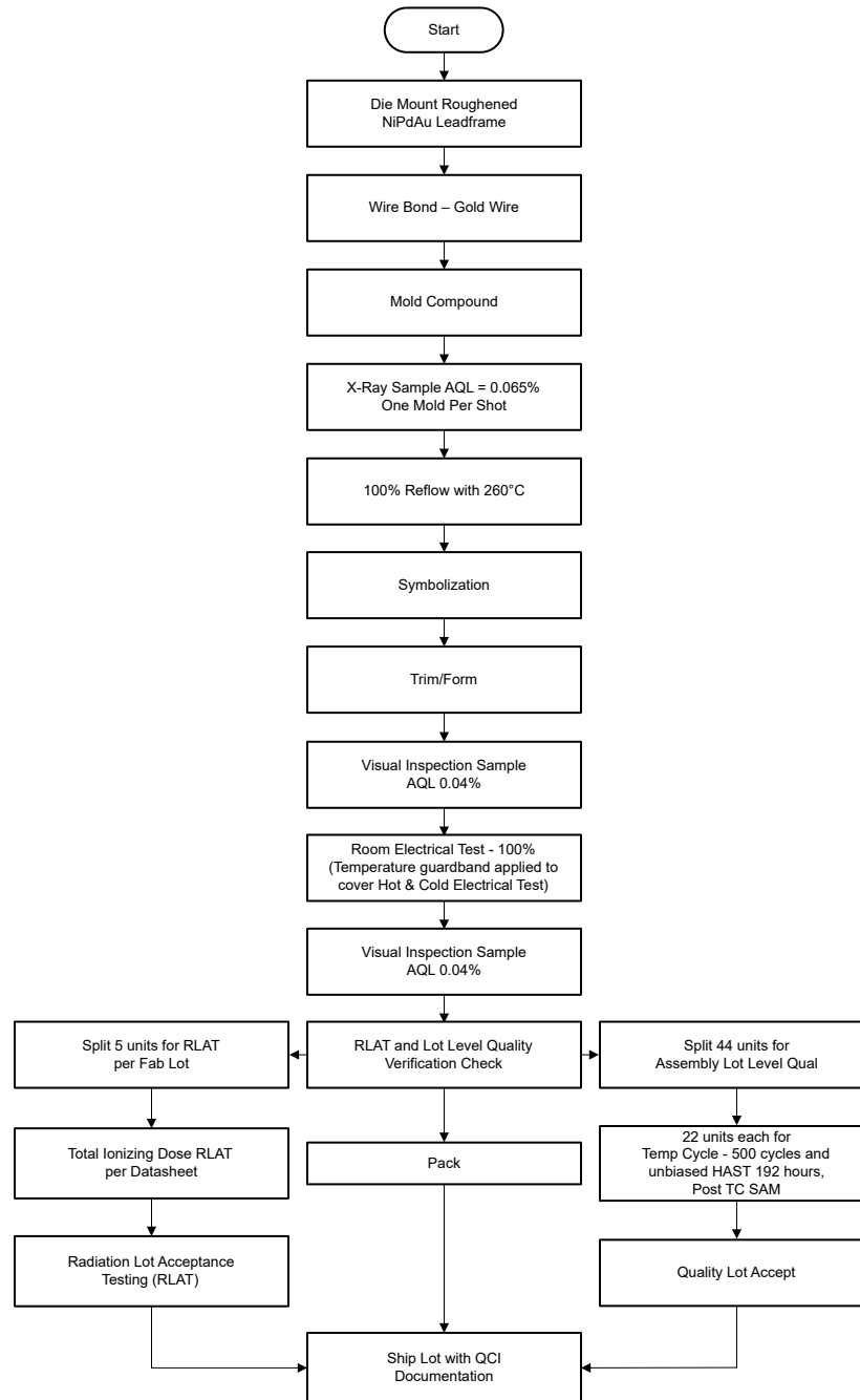
Figure 1-1. SN54SC1G125-SEP Space Enhanced Plastic Production Flow Chart
