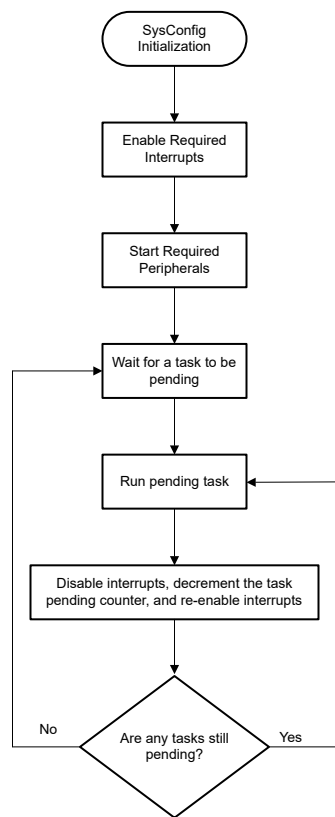
Figure 5-1. Application Software Flow Chart
