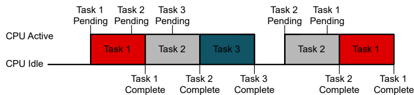
Figure 1-1. Run-to-Completion Scheduler
