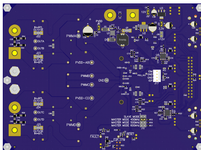
Figure 3. EVM Board (Bottom Side)
