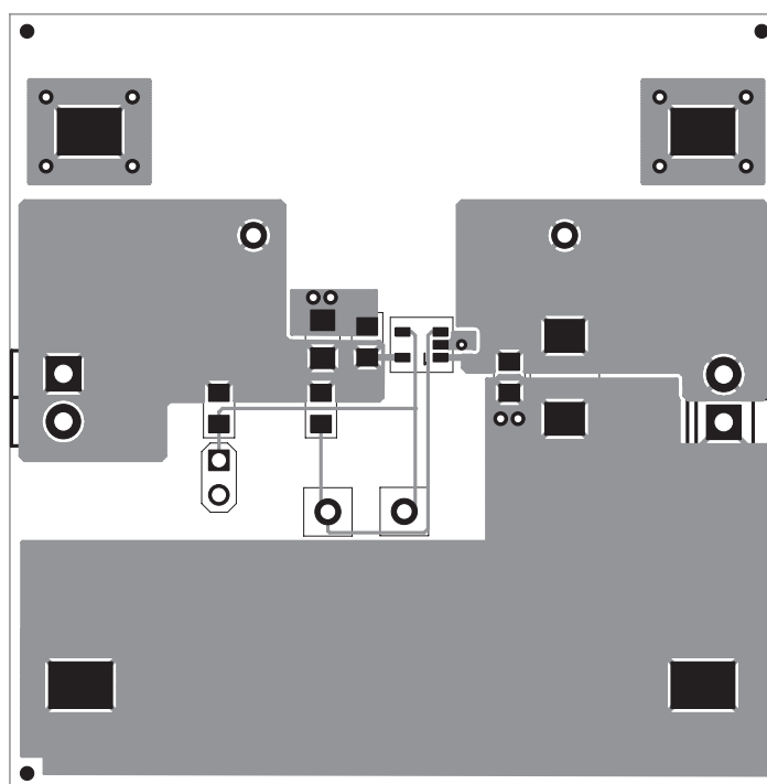
Figure 4. TPS20xxCDBVEVM-636 Top-Side Layout
