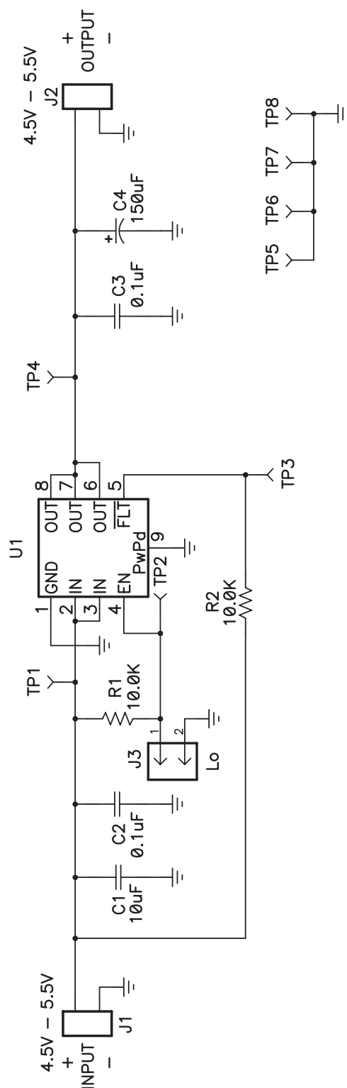
Figure 2. TPS20xxCDGNEVM-635 Schematic
