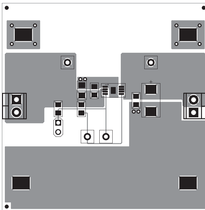
Figure 7. TPS20xxCDGNEVM-635 Top-Side Layout
