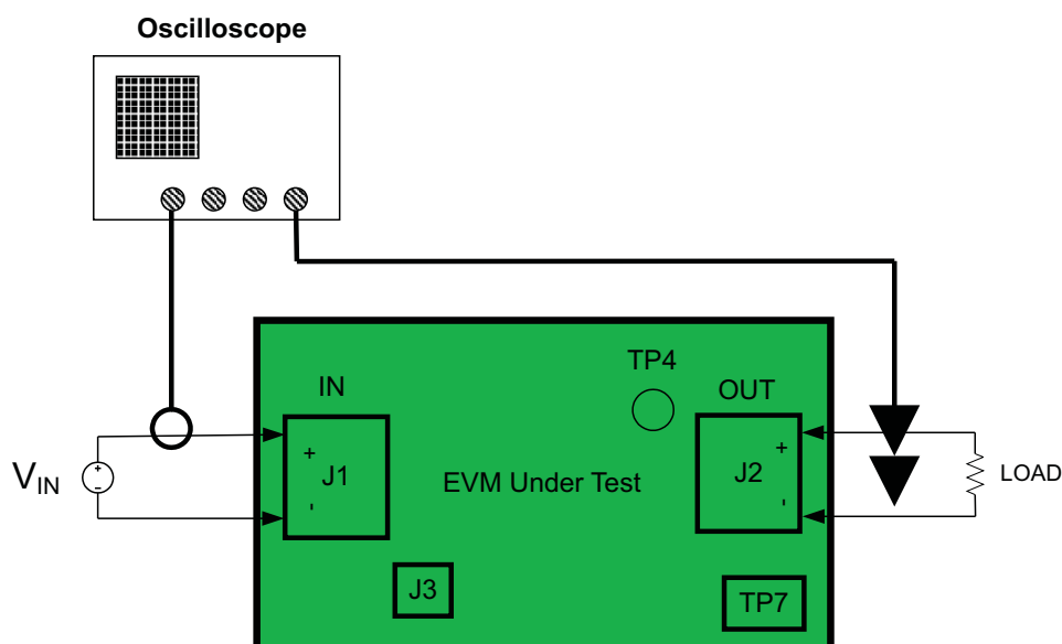
Figure 9. EVM Setup For Measuring Current Limit
