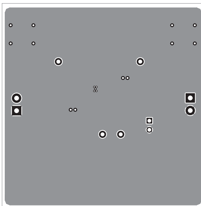
Figure 8. TPS20xxCDGNEVM-635 Bottom-Side Layout
