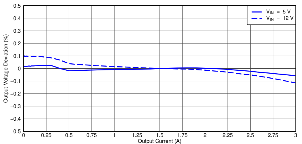
Figure 4-3. TPS54329EVM-056 Load Regulation, V_{IN} = 5V
