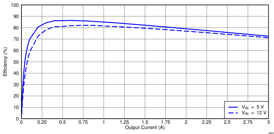
Figure 4-1. TPS54329EVM-056 Efficiency
