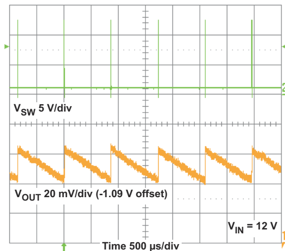
Figure 4-10. TPS54428EVM-052 Eco-mode™ Output Voltage Ripple at No Load
