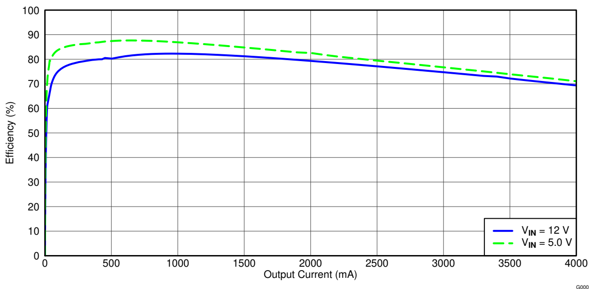
Figure 4-1. TPS54428EVM-052 Efficiency
