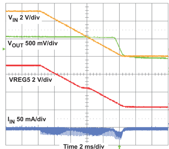
Figure 4-13. TPS54428EVM-052 Shut-down Relative to V_{IN}
