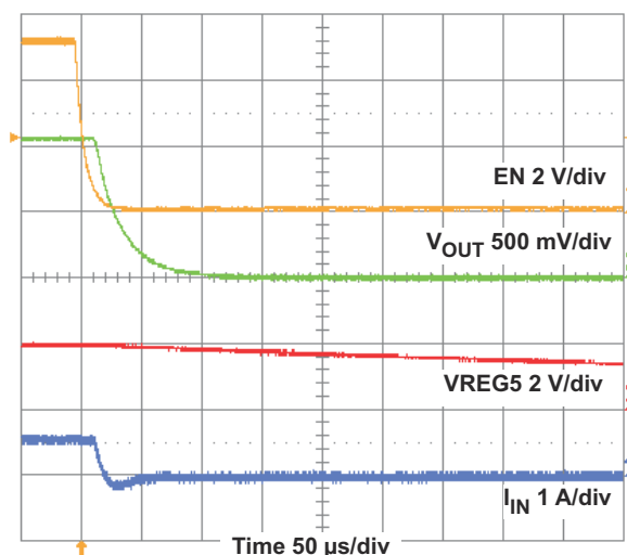
Figure 4-15. TPS54428EVM-052 Shut-down Relative to EN
