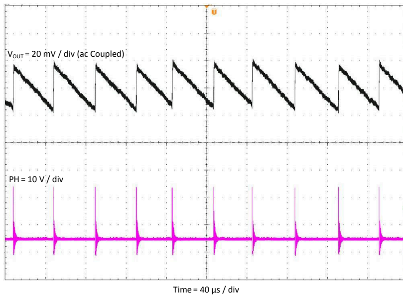
Figure 2-8. TPS54302EVM-716 Output Ripple, I_{OUT} = 10 mA
