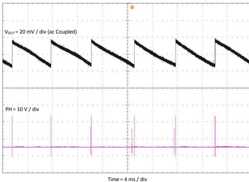
Figure 2-9. TPS54302EVM-716 Output Ripple, I_{OUT} = 0 A
