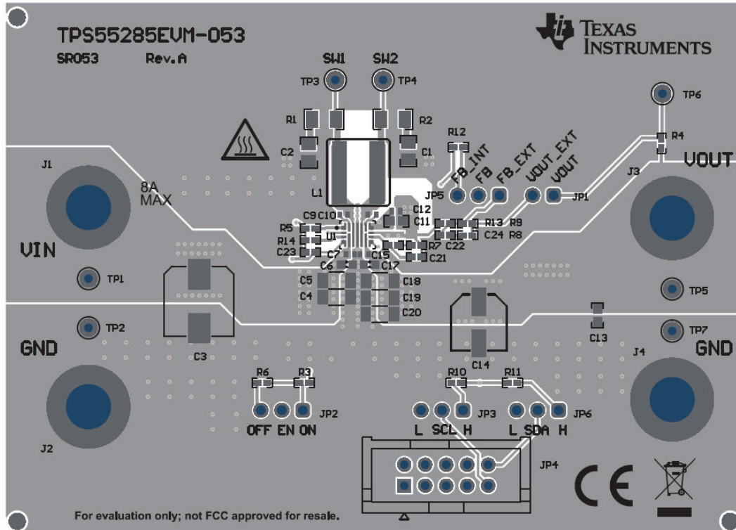
Figure 4-2. TPS55285EVM-053 Top-Side Layout
