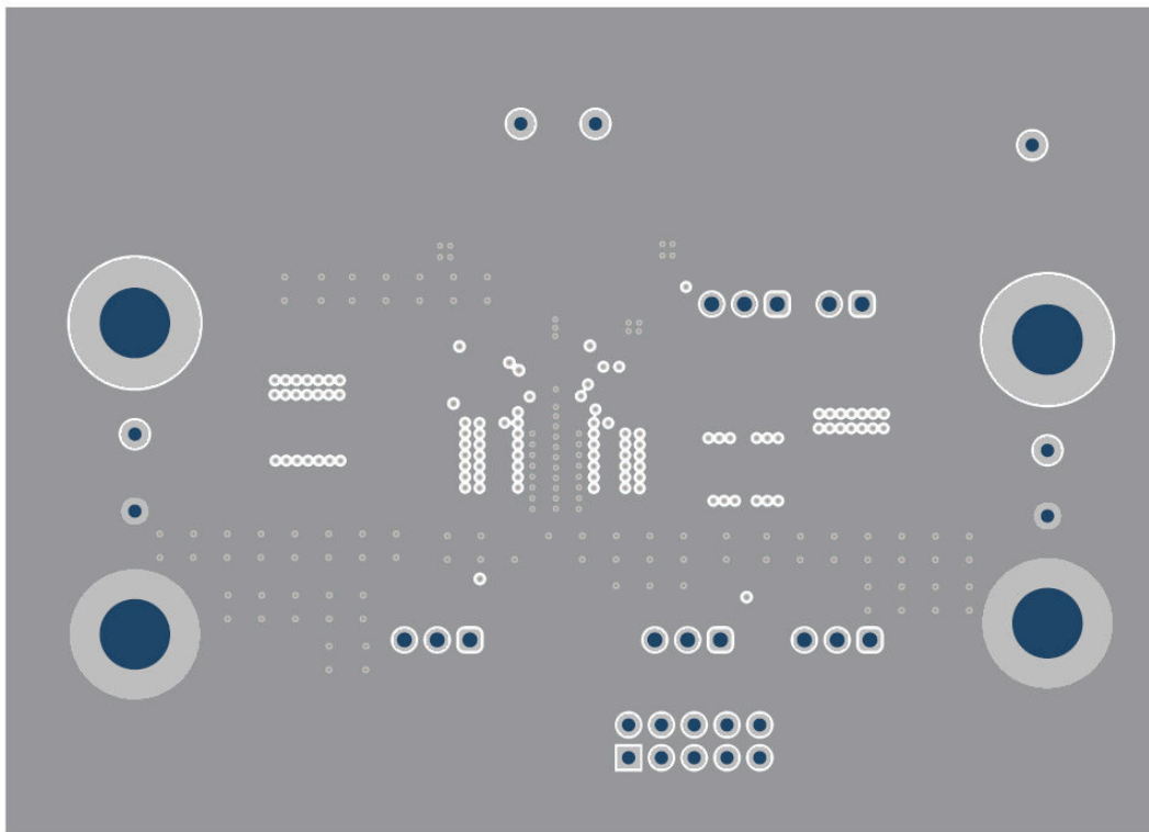
Figure 4-3. TPS55285EVM-053 Inner Layer1
