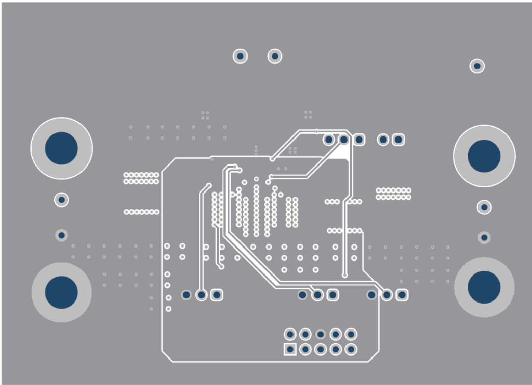
Figure 4-4. TPS55285EVM-053 Inner Layer2
