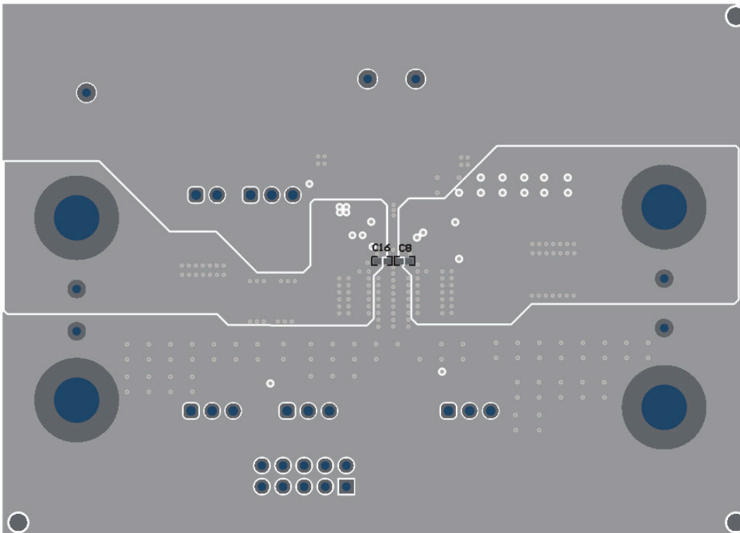
Figure 4-5. TPS55285EVM-053 Bottom-Side Layout
