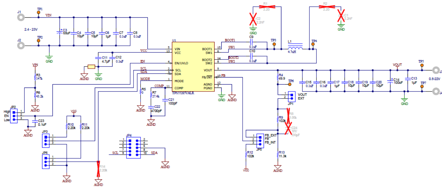
Figure 4-1. TPS55285EVM-053 Schematic
