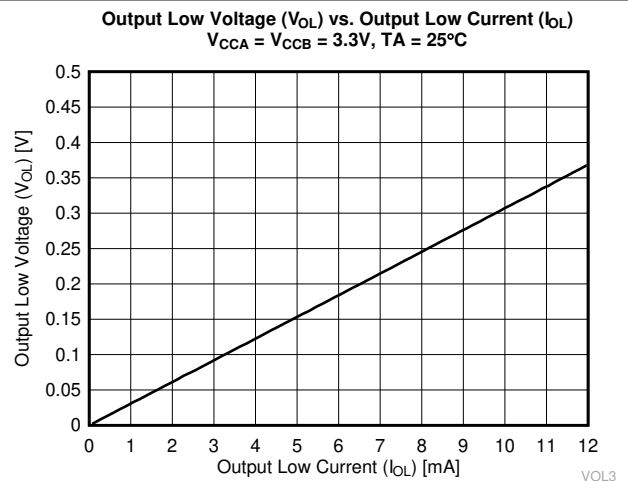
Figure 5-6. V_{OL} vs I_{OL} , 3.3 V
