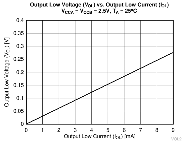
Figure 5-4. V_{OL} vs I_{OL} , 2.5 V
