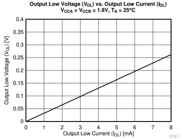
Figure 5-2. V_{OL} vs I_{OL} , 1.8 V
