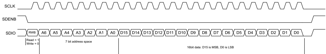
Figure 41. Serial Register Write Timing Diagram
