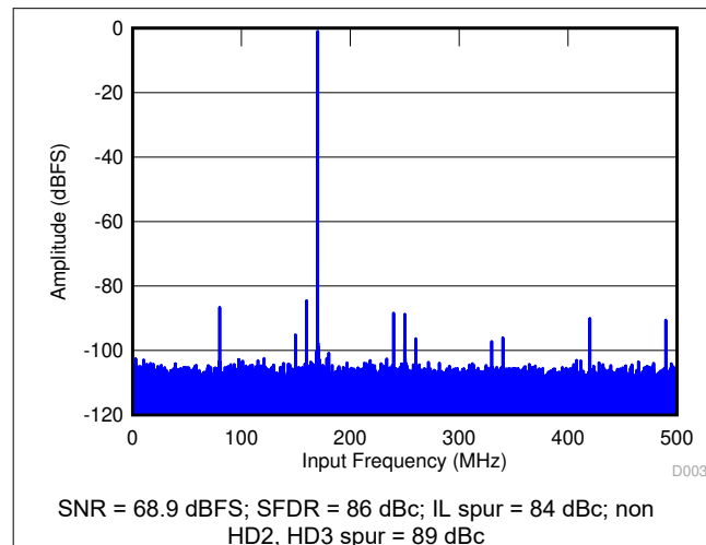
Figure 9-18. FFT for 170-MHz Input Signal
