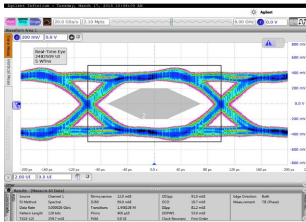
Figure 8-23. Eye at 5-Gbps Bit Rate with Default Output Swing
