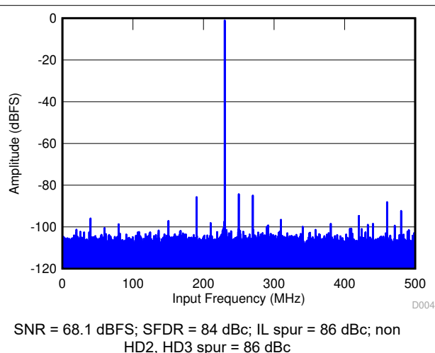
Figure 9-19. FFT for 230-MHz Input Signal
