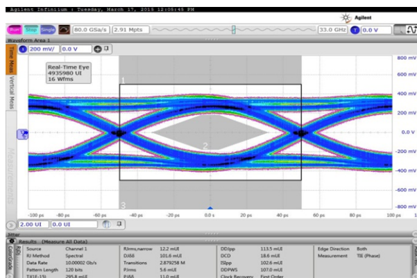
Figure 8-25. Eye at 10-Gbps Bit Rate with Default Output Swing
