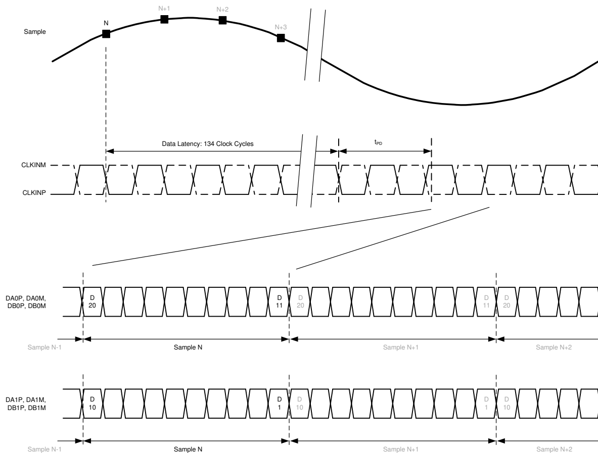
Figure 7-2. Sample Timing Requirements
