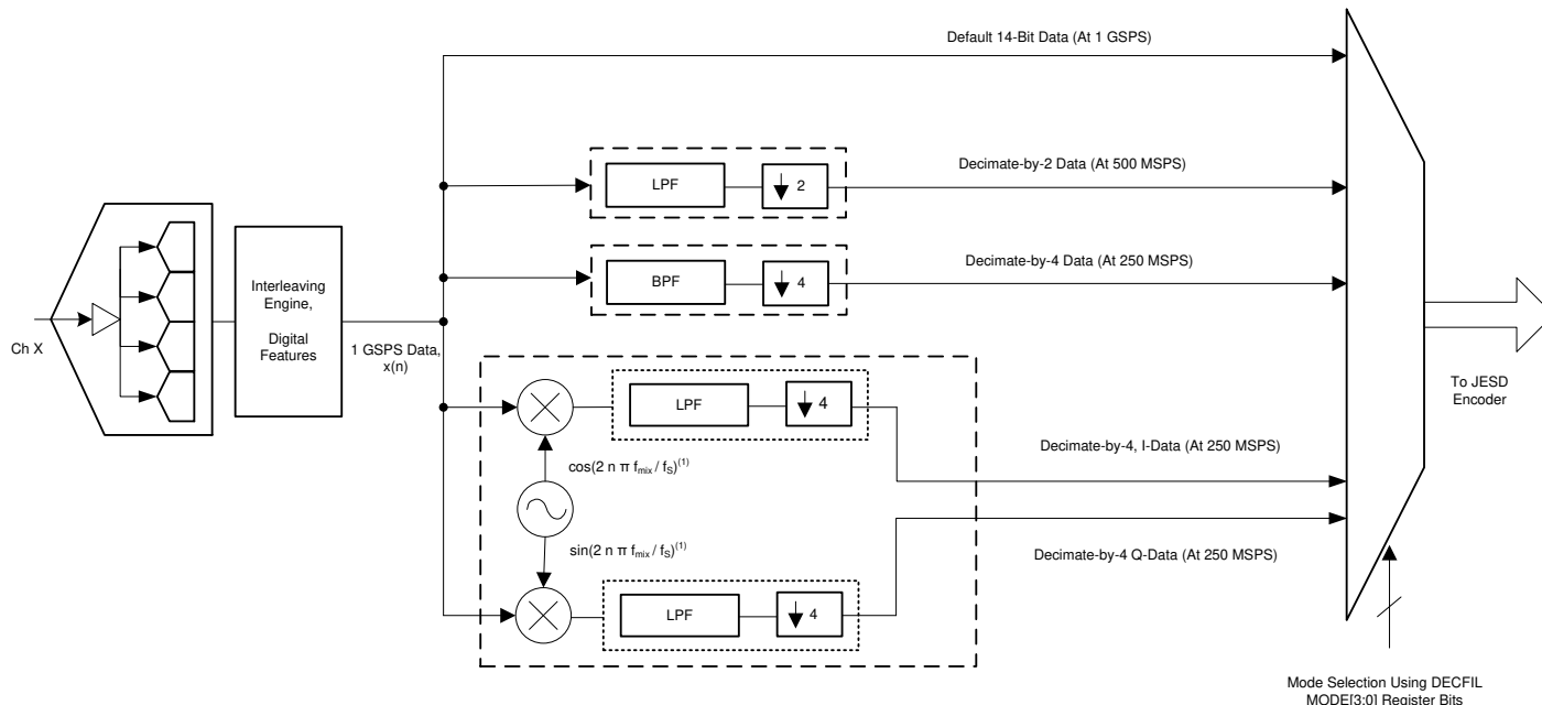
Figure 8-3. DDC Block
