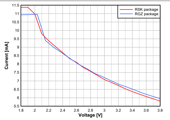
Figure 8-13. TX Current vs. Supply Voltage (VDD5) (BLE 1 Mbps, 2.44 GHz, 0 dBm)
