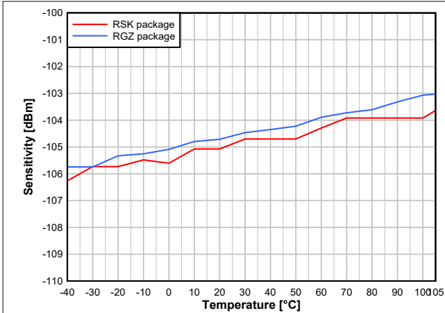
Figure 8-20. Sensitivity vs. Temperature (250 kbps, 2.44 GHz)
