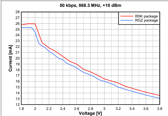
Figure 8-12. TX Current vs. Supply Voltage (VDD5) (50 kbps, 868.3 MHz)
