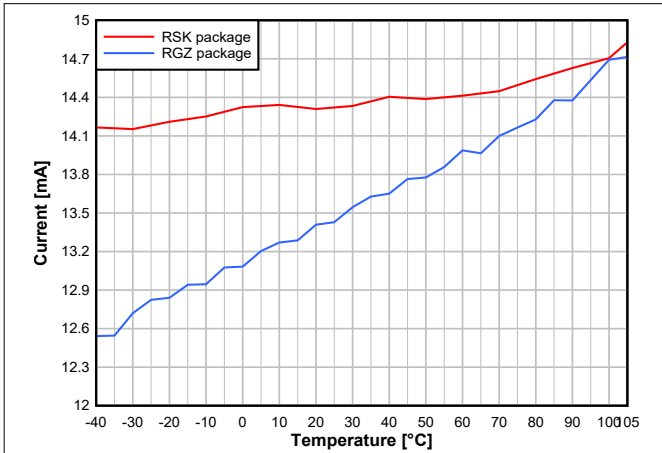
Figure 8-10. TX Current vs. Temperature (50 kbps, 868.3 MHz, +10 dBm, VDD5 = 3.6 V)
