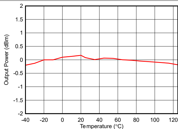
Figure 7-22. Output Power vs Temperature (BLE 1Mbps, 2.44GHz, 0dBm)
