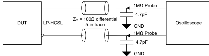
Figure 6-1. Regular LP-HCSL Test Load
