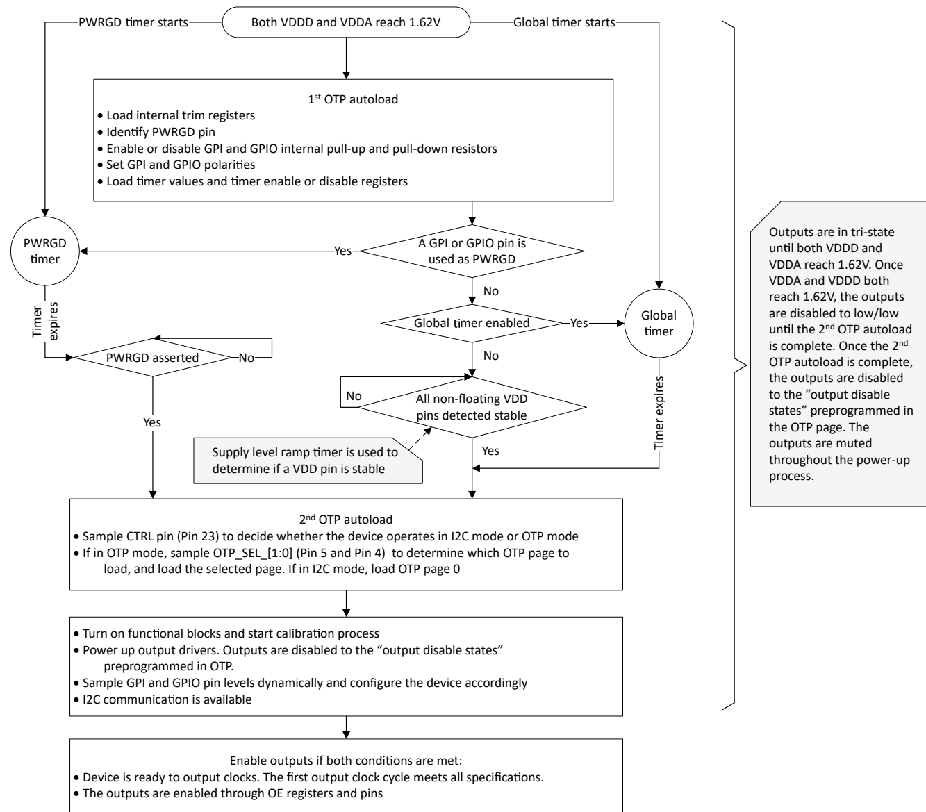
Figure 7-4. LMK3H2104 Power Up Sequence
