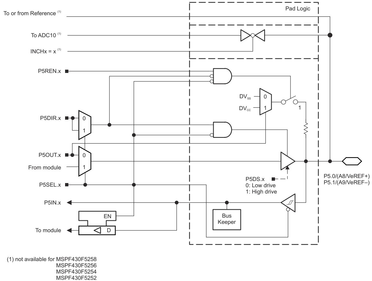
Figure 9-6. Port P5 (P5.0 and P5.1) Diagram
