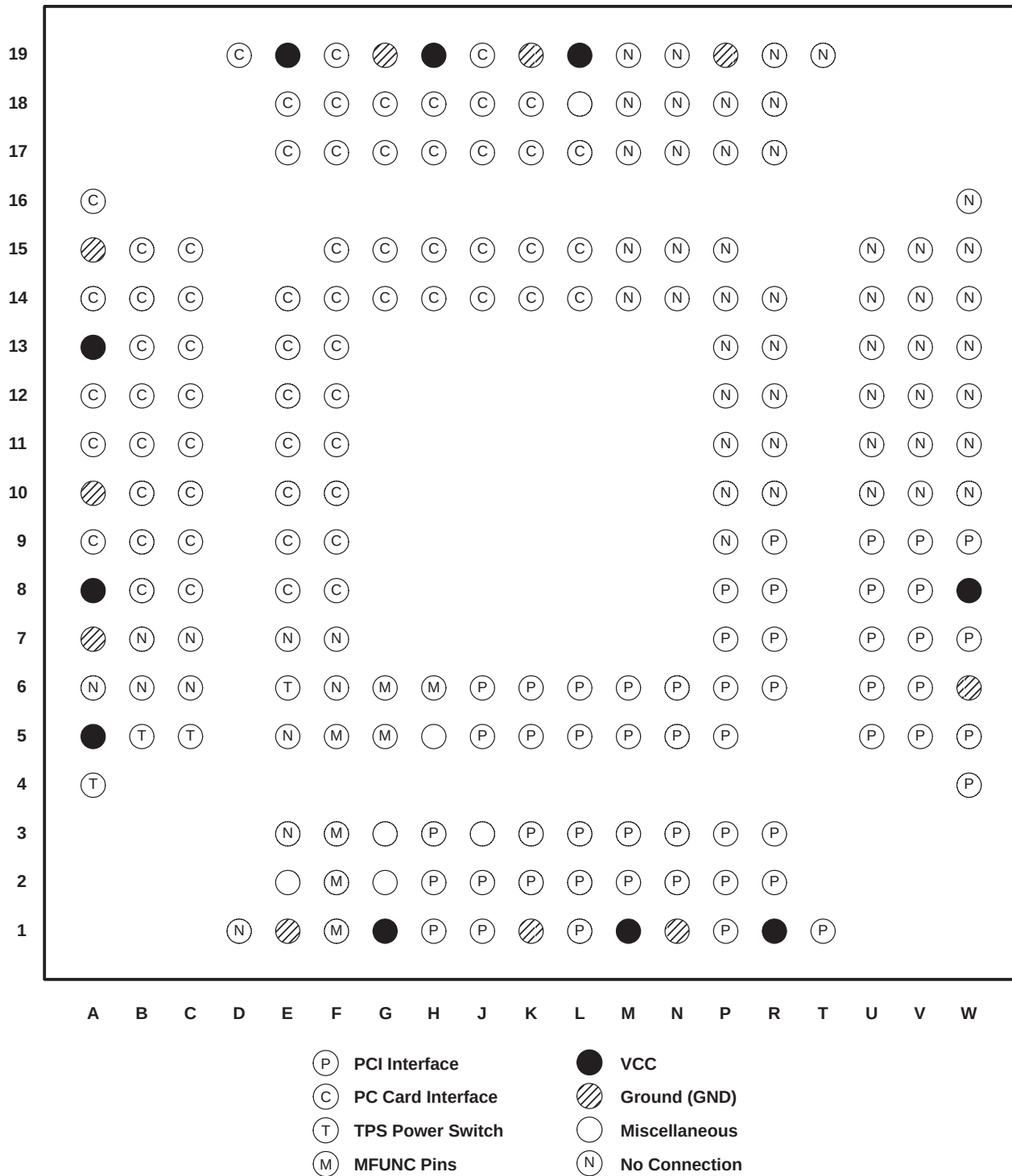
Figure 2-2. PCI1510 GVF-Package Terminal Diagram
