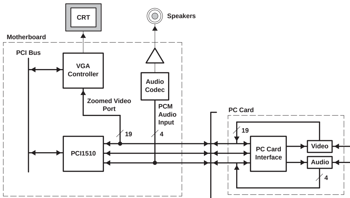
Figure 3-4. Zoomed Video Implementation Using the PCI1510 Controller
