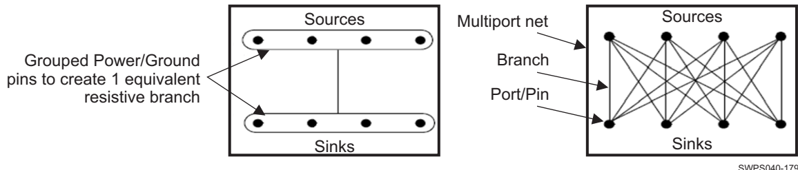
Figure 7-11. Pin-grouping concept: Lumped and Distributed Methodologies
