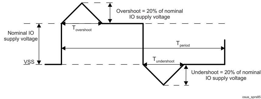
Figure 5-1. T_{\text{overshoot}} + T_{\text{undershoot}} < 20\% \text{ of } T_{\text{period}}
