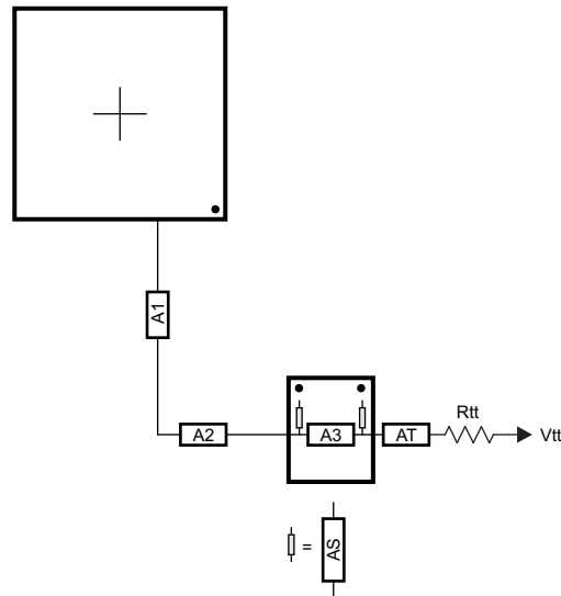
Figure 7-70. ADDR_CTRL Routing for Two Mirrored DDR3 Devices
