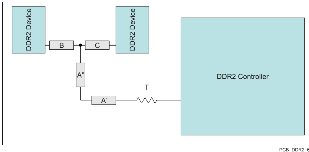
Figure 7-52. CK and ADDR_CTRL Routing and Topology
