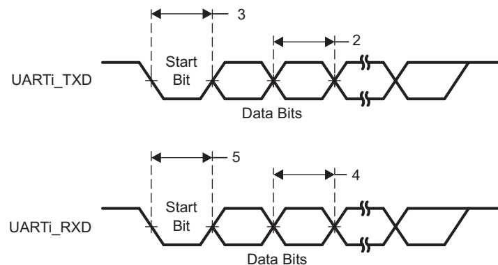
Figure 5-41. UART Timing
