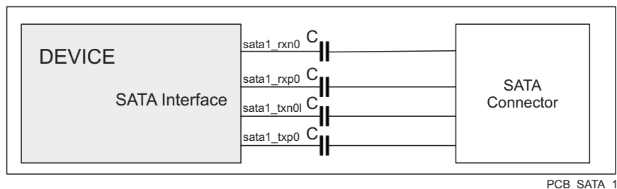
Figure 7-45. SATA Interface High Level Schematic
