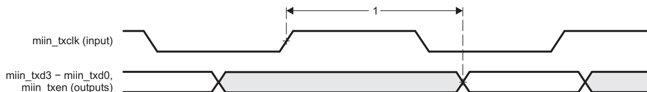
Figure 5-64. GMAC Transmit Interface Timing MII n Operation
