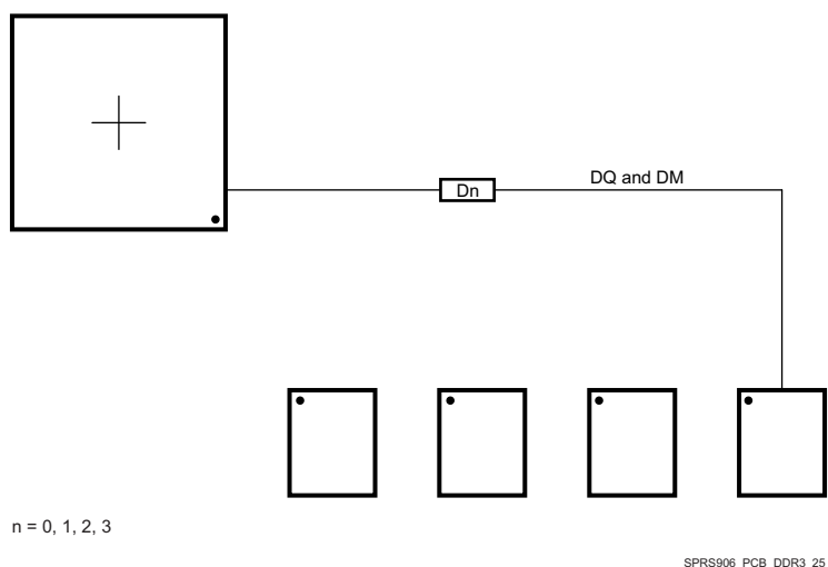
Figure 7-78. DQ/DM Routing With Any Number of Allowed DDR3 Devices
