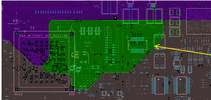
Figure 7-23. vdd_mpu routing [Internal Power Plane #2]
