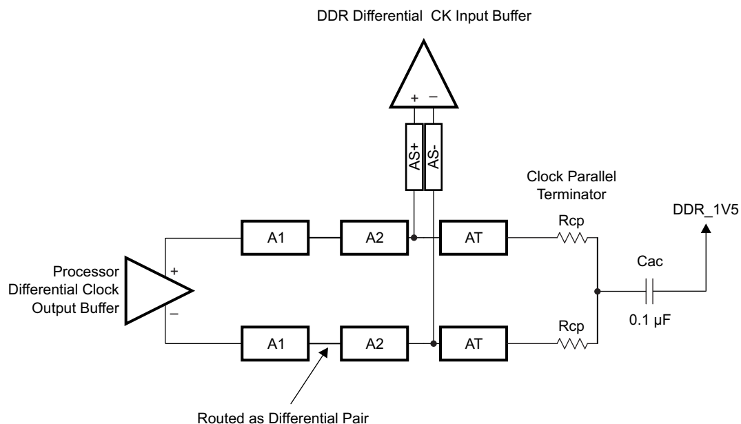
Figure 7-71. CK Topology for One DDR3 Device
