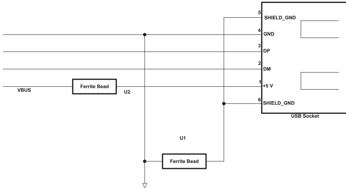
Figure 7-32. USB Connector
