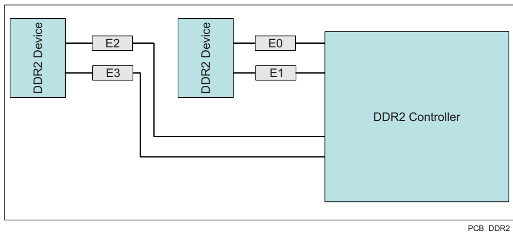
Figure 7-53. DQS and DQ Routing and Topology
