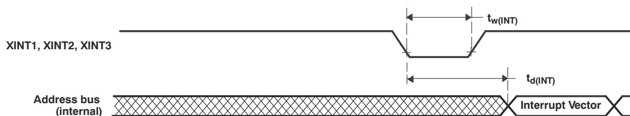
Figure 9-15. External Interrupt Timing
