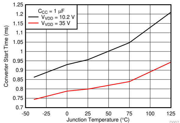
Figure 6-6. Converter Startup Time vs Temperature
