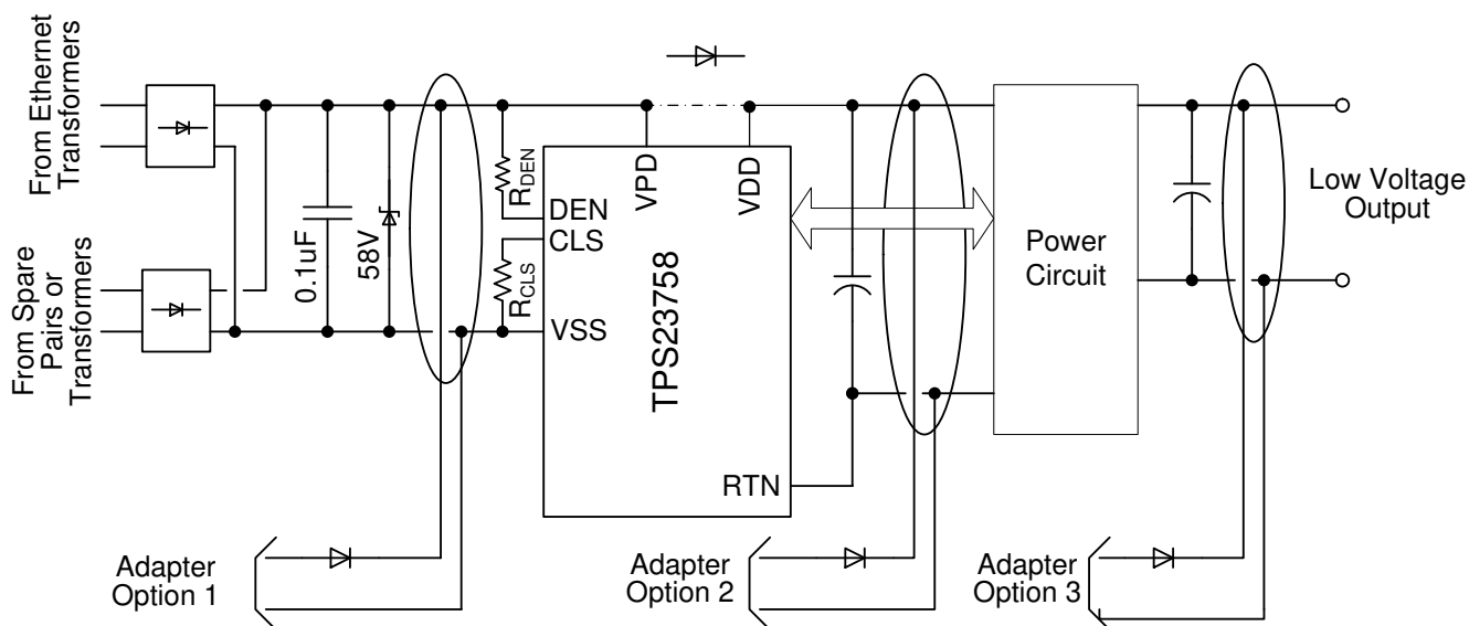
Figure 7-10. ORing Configurations
