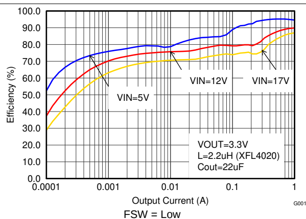
Figure 16. Efficiency versus Output Current
