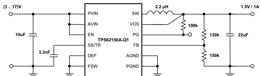
Figure 47. 1.5-V/1-A Power Supply
