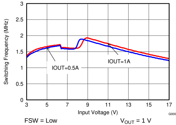
Figure 30. Switching Frequency versus Input Voltage
