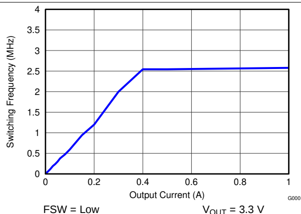
Figure 27. Switching Frequency versus Output Current
