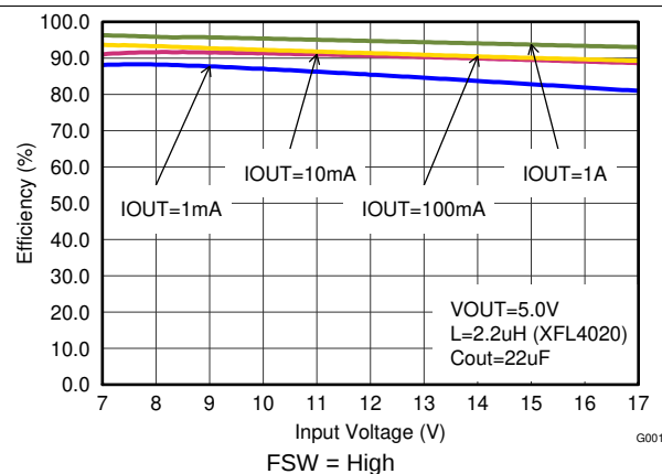
Figure 15. Efficiency versus Input Voltage
