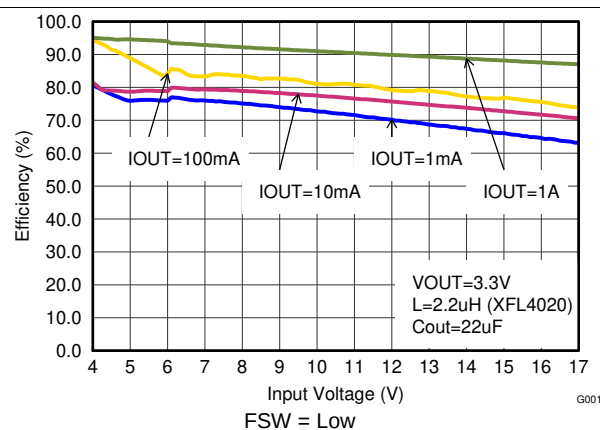
Figure 17. Efficiency versus Input Voltage
