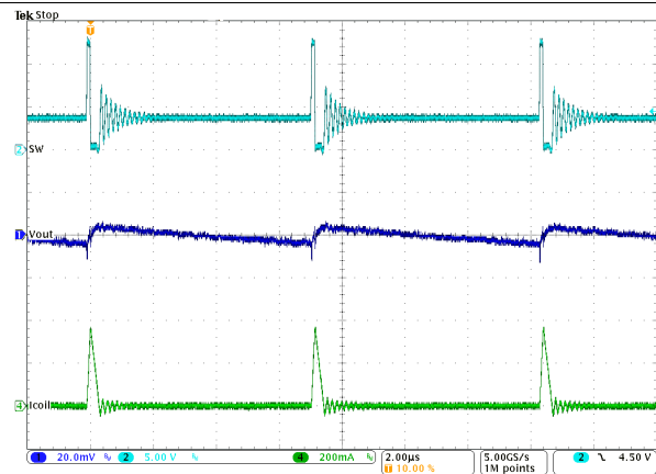
Figure 33. Typical Operation in Power Save Mode ( I_{OUT} = 10 mA)
