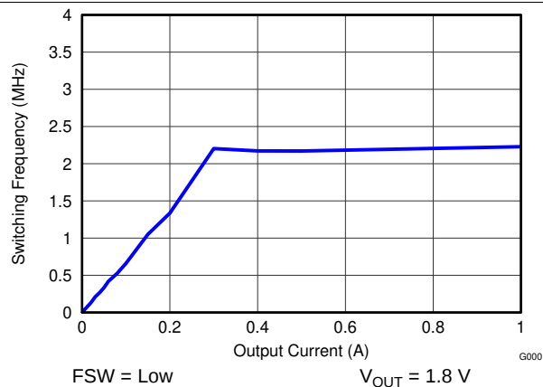
Figure 29. Switching Frequency versus Output Current
