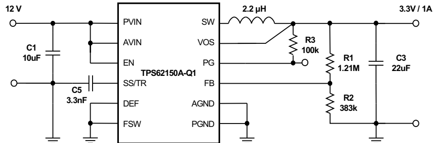
Figure 9. Typical Schematic for 3.3-V Step-Down Converter
