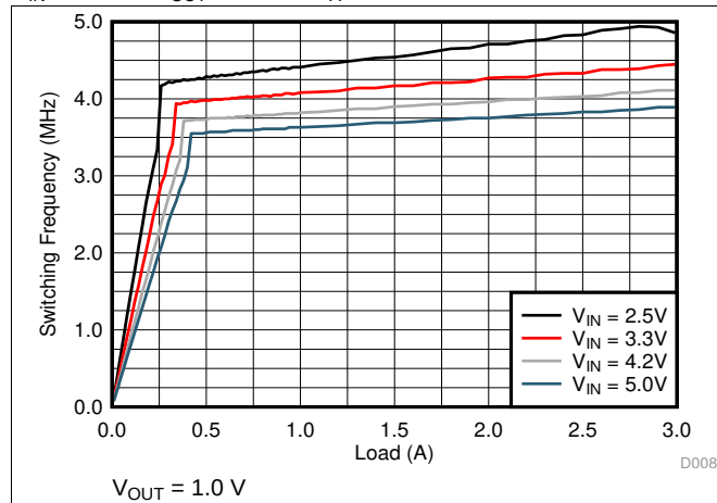
Figure 8. Switching Frequency
