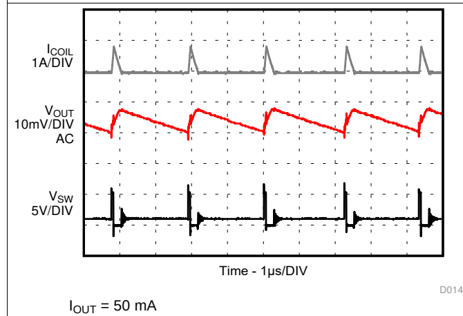
Figure 10. PSM Operation
