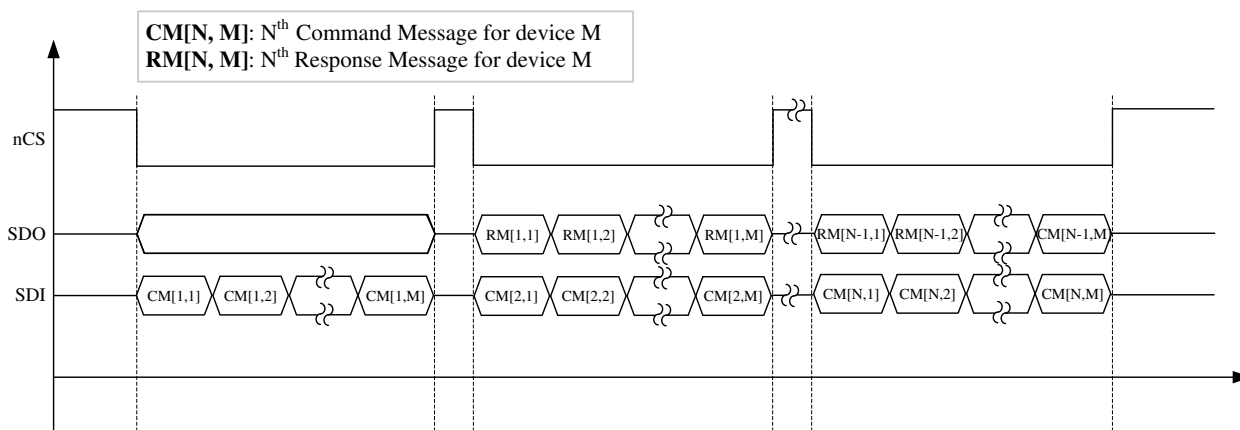
Figure 7-41. SPI message frame daisy chain SPI configuration
