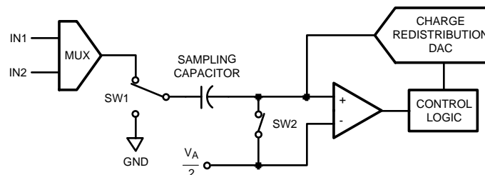
Figure 48. ADC102S051 in Track Mode
