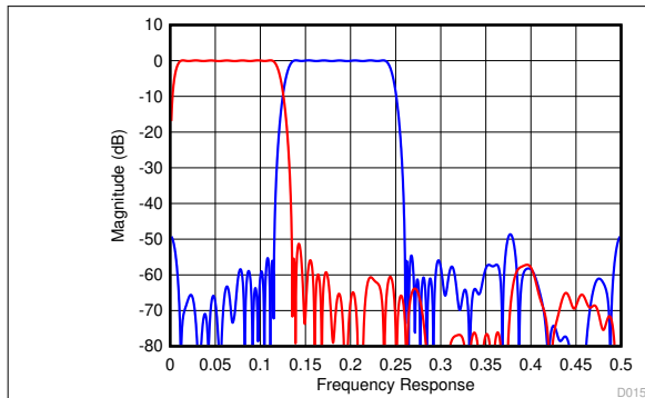
8-6. Decimate-by-4 Filter Response
