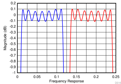
8-7. Decimate-by-4 Filter Response (Zoomed)
