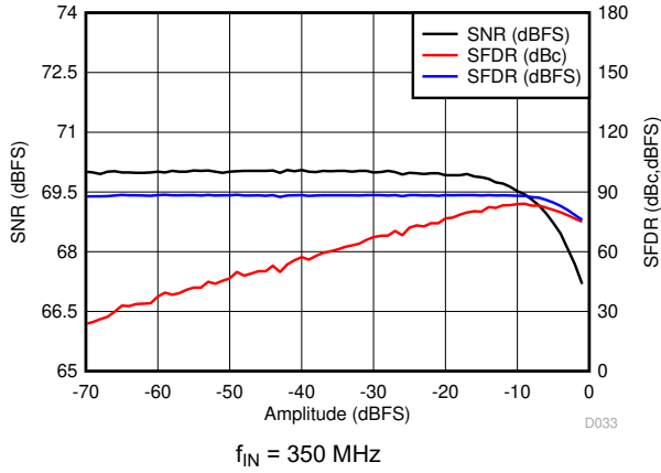
7-39. Performance vs Input Amplitude
